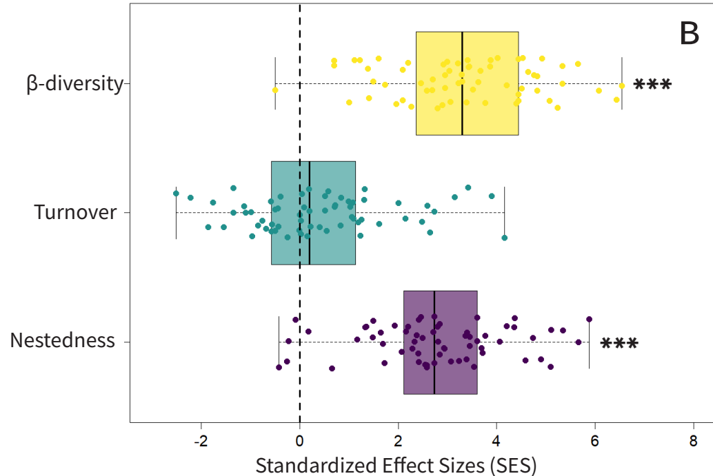
(b) Functional beta diversity
