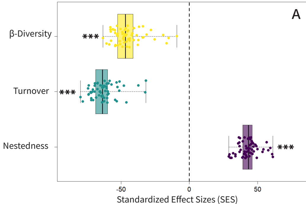
(a) Taxonomic beta diversity
